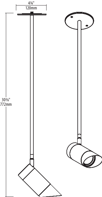
With oval snoot and 2' rod
