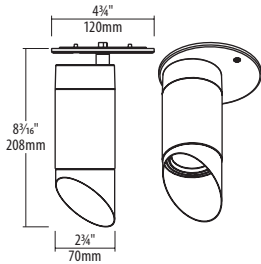
With oval snoot
