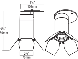
With barn door
