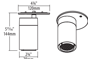
With honeycomb louver
