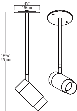
With snoot and 1' rod
