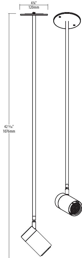
With honeycomb louver and 3' rod
